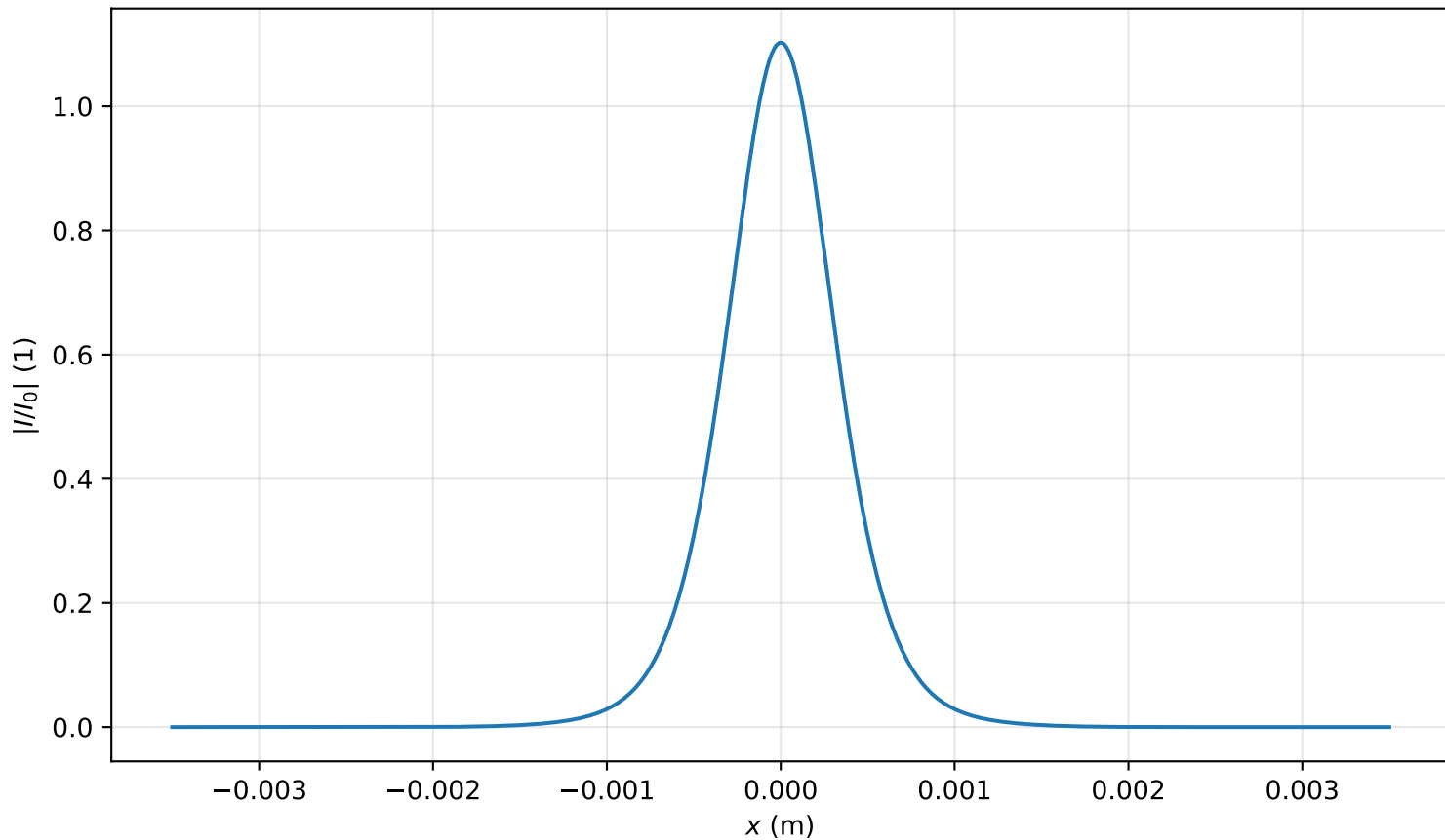
Intensity profile I(x, y = 0, z = 1.990m)/I_0 , P_{in}=0.7P_{cr} , artificial time
